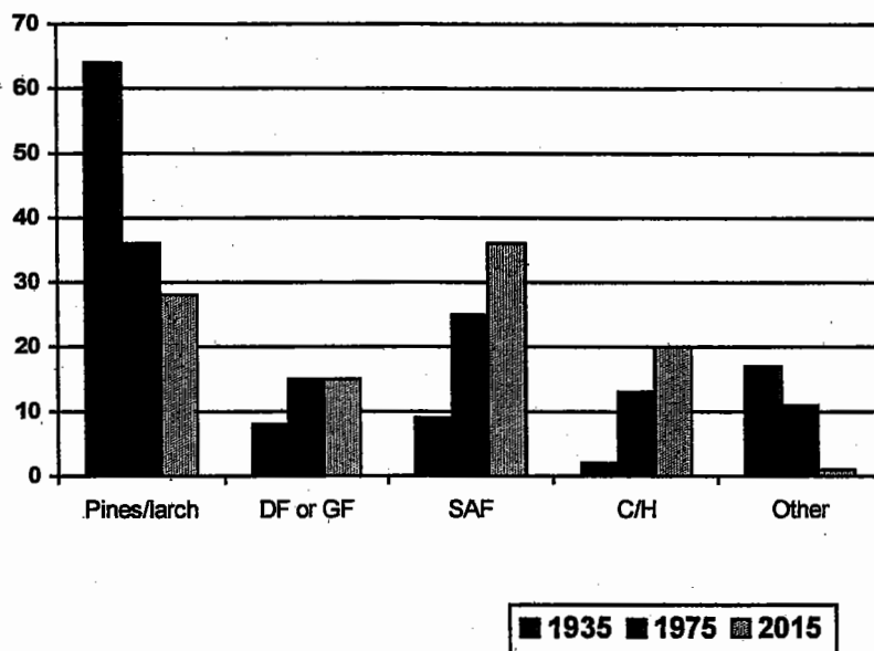
Figure 1: Changes in cover type in M333d from 1935 to 1975 and predicted through 2015.
